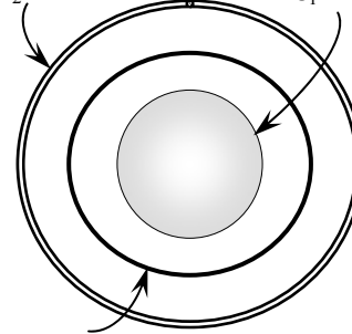
Radiation shield D_3 = 0.2 \text{ m} \varepsilon_3 = 0.2
